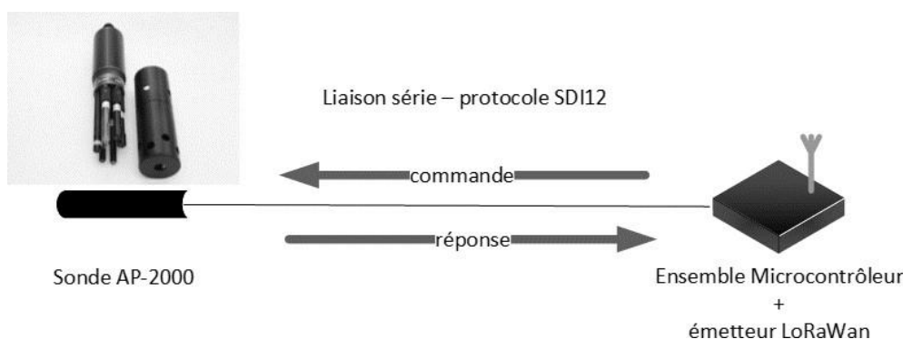
Figure 3: communication SDI12
